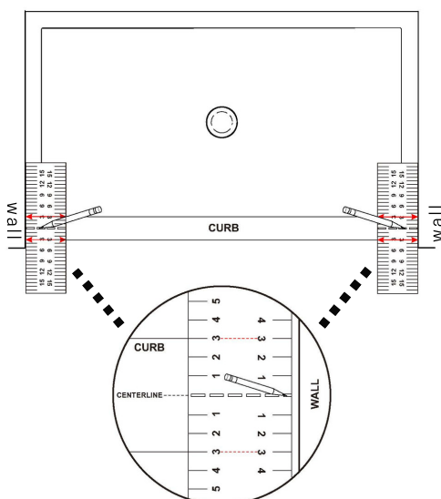
Engineered templates easily determines hardware placement
